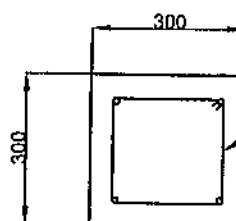
PEDESTAL PLAN
