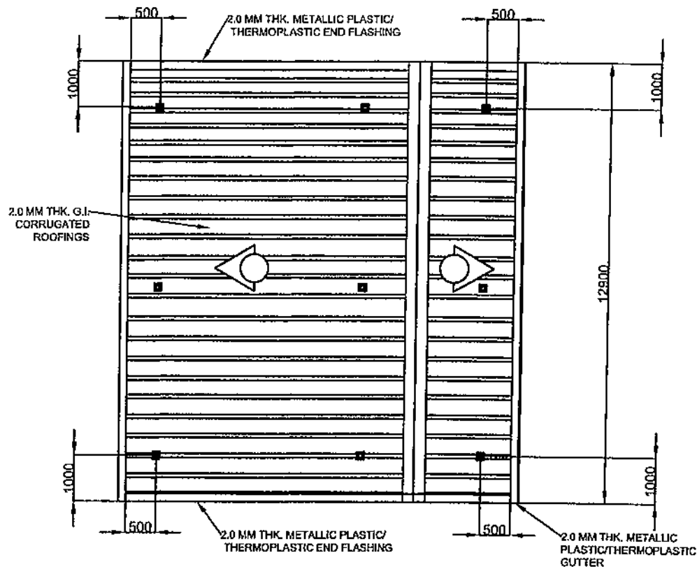
ROOFING DETAILS
