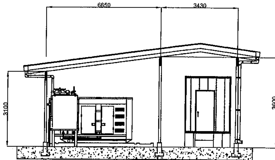
SIDE VIEW
